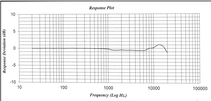
Typical free-field response of the microphone with the grid cap at 0 degree incidence. The corrected free-field curve is shown.
